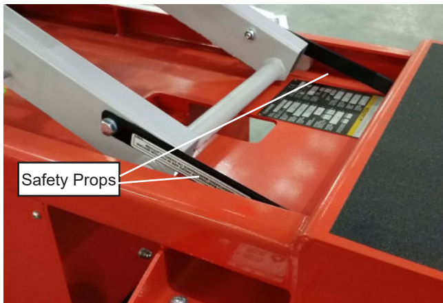
Figure 5 – Safety Props
