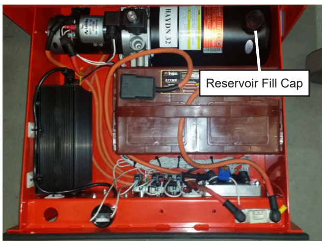
Figure 6 – Component Tray
